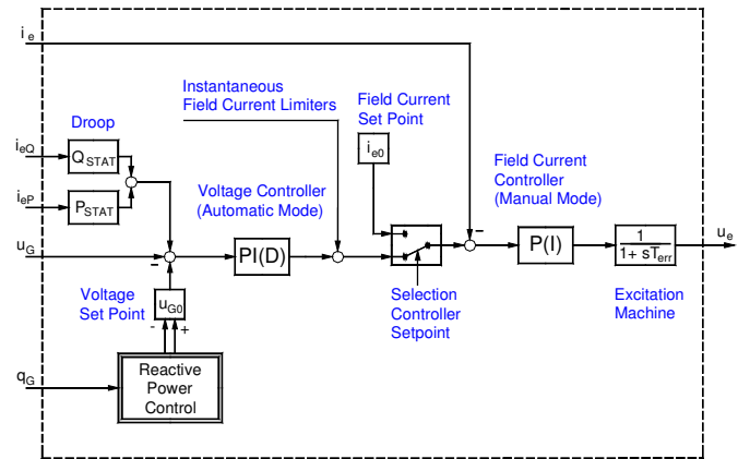
Fig. 6. Block diagram of voltage regulator ELIN GMR3 in PSP Markersbach
