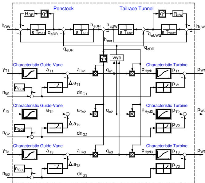
Fig. 4. Block diagram of the hydraulic and mechanical sub-model of a partial plant
