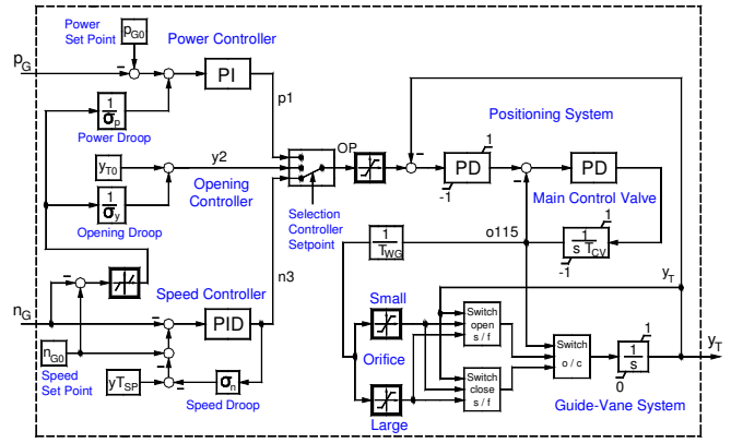
Fig. 5. Block diagram of turbine regulator Sulzer DTL 595 (Francis) in PSP Markersbach
